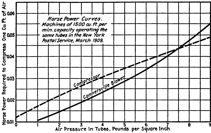
FIG. 25.—Power consumed by rotary and piston compressor.
